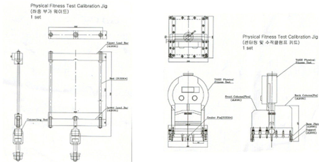
Supplementary Fig. 1. Jig production drawings for calibration.
